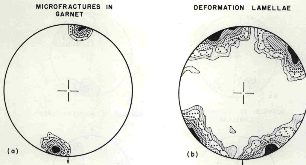
Fig. 41—Diagrams illustrating the orientation of microfractures in garnet (a) and deformation lamellae in quartz (b) (from Naha, Ref. 149, Fig. 2). Plane of each diagram is parallel to the ac plane of a fold, i.e., the fold axis is at the center. (a) Normals to 54 microfractures in 14 garnet grains. Contours are at 5, 10, 20, 30, 40, and 45 per cent per 1 per cent area, 52 per cent maximum. (b) Normals to 158 deformation lamellae in quartz. Contours are at 0.66, 1.3, 3.5, 7, 9, and 11 per cent per 1 per cent area, 13.7 per cent maximum.
