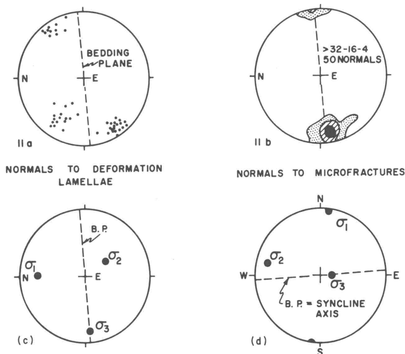
Fig. 40—Diagrams (11a and 11b) illustrating the orientation of 50 sets of quartz deformation lamellae and of microfractures, respectively, in a Baraboo quartzite specimen (from Riley, Ref. 141, Fig. 11). (c) Stereogram shows the orientation of the principal stresses deduced from the deformation lamellae and the microfractures, assuming the latter are extension fractures and the former are in planes of high shear stress and inclined at < 45 degrees to \sigma_1 . (d) Stereogram shows same data rotated to horizontal plane, with north as indicated. \sigma_1 is nearly perpendicular to both the synclinal axis and the bedding plane.
